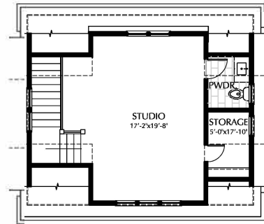
GARAGE SECOND FLOOR PLAN
