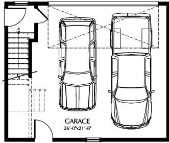
GARAGE FLOOR PLAN
